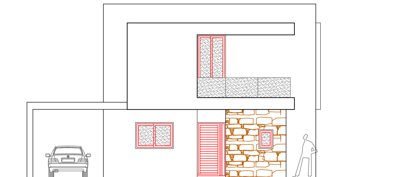
Entrance elevation
