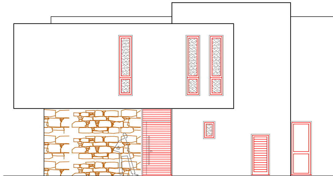
Entrance elevation
